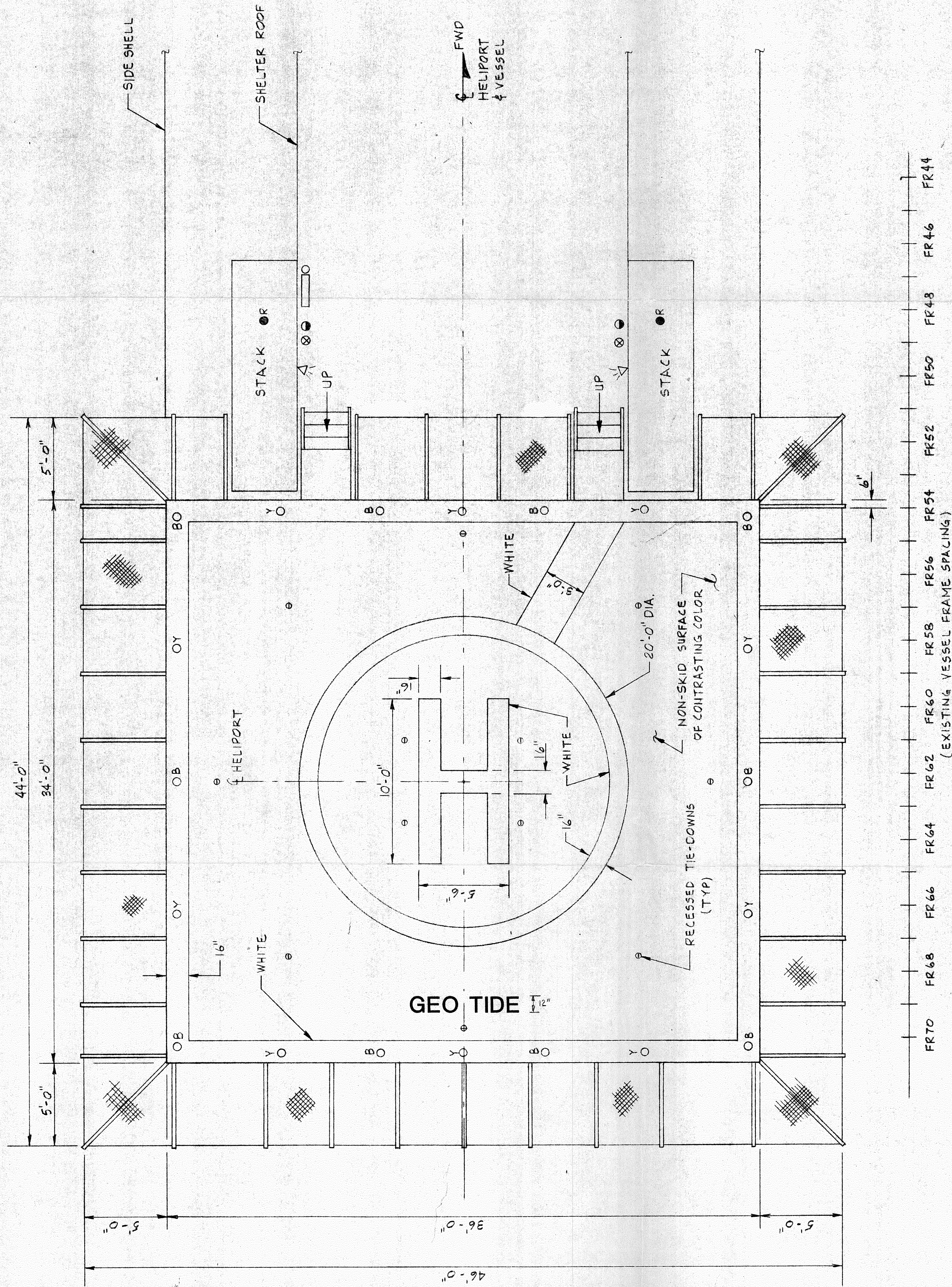
PLAN OF HELIDECK SCALE: 1/4" = 1'-0"
